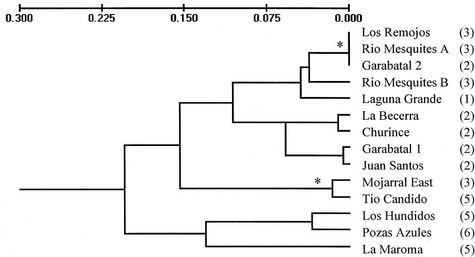
Figure 3. UPGMA dendrogram of Nei's genetic distance (Nei, 1978) between populations. Drainage numbers for each site are in parenthesis. * (asterisks) designate the two nodes with consistently high bootstrap values (65–85%) that are discussed in the text.
